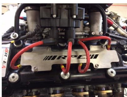
Individual Throttle Body Adjustment
