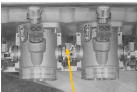
Individual Throttle Body Adjustment
